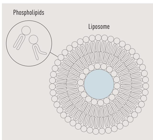
Fig. 1: Schematic diagram of phospholipids and a liposome
